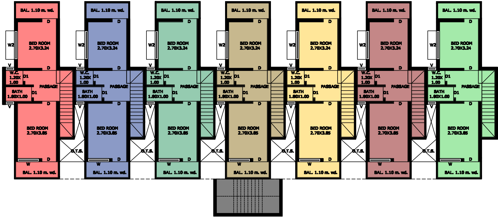
THIRD FLOOR PLAN (BUILDING-"A")
