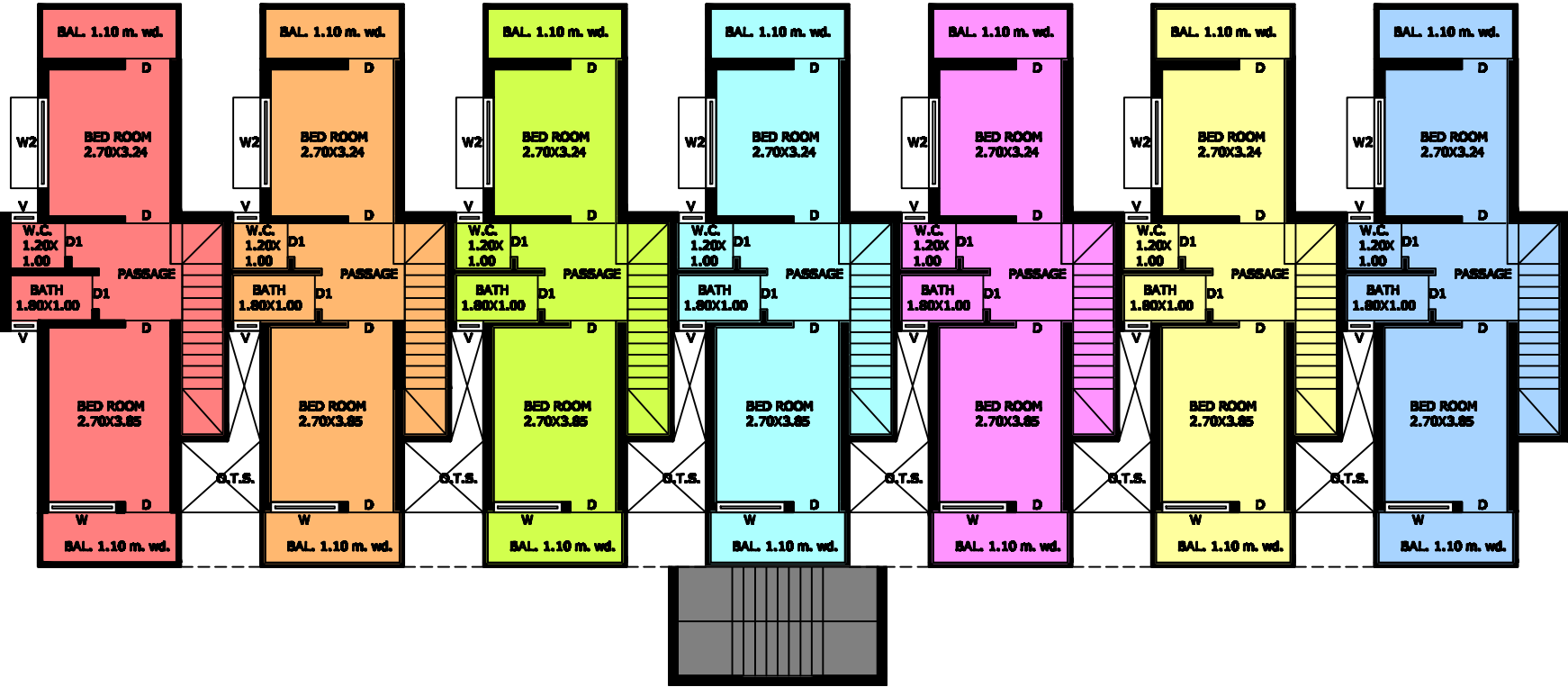
FIRST FLOOR PLAN (BUILDING-"A")
